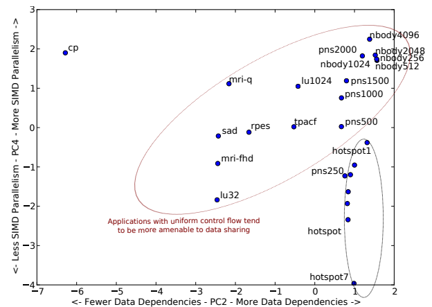
Figure 7: A comparison between Control Flow Divergence and Data Dependencies/Sharing. Excluding the hotspot applications, applications with more uniform control flow exhibit a greater degree of data sharing among threads. Well structured algorithms that benefit from low control flow divergence and include mechanisms for fine grained inter-thread communication.
