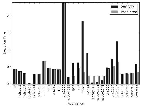
Figure 9: Predicted execution times for the 280GTX using only static data. The left 12 applications are used to train the model and the predictions are made for the rightmost 13 applications.
