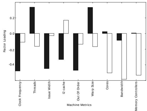
Figure 3: Factor loadings for two machine principal components. PC0 (black) corresponds to single core performance, while PC1 (white) corresponds to multi-core throughput.
