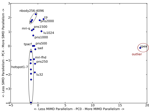
Figure 6: This plot compares MIMD to SIMD parallelism. It should be clear that these metrics are completely independent for this set of applications; the fact that an application can be easily mapped onto a SIMD processor says nothing about its suitability for a multi-core system. A complementary strategy may be necessary that considers both styles of parallelism when designing new applications.
