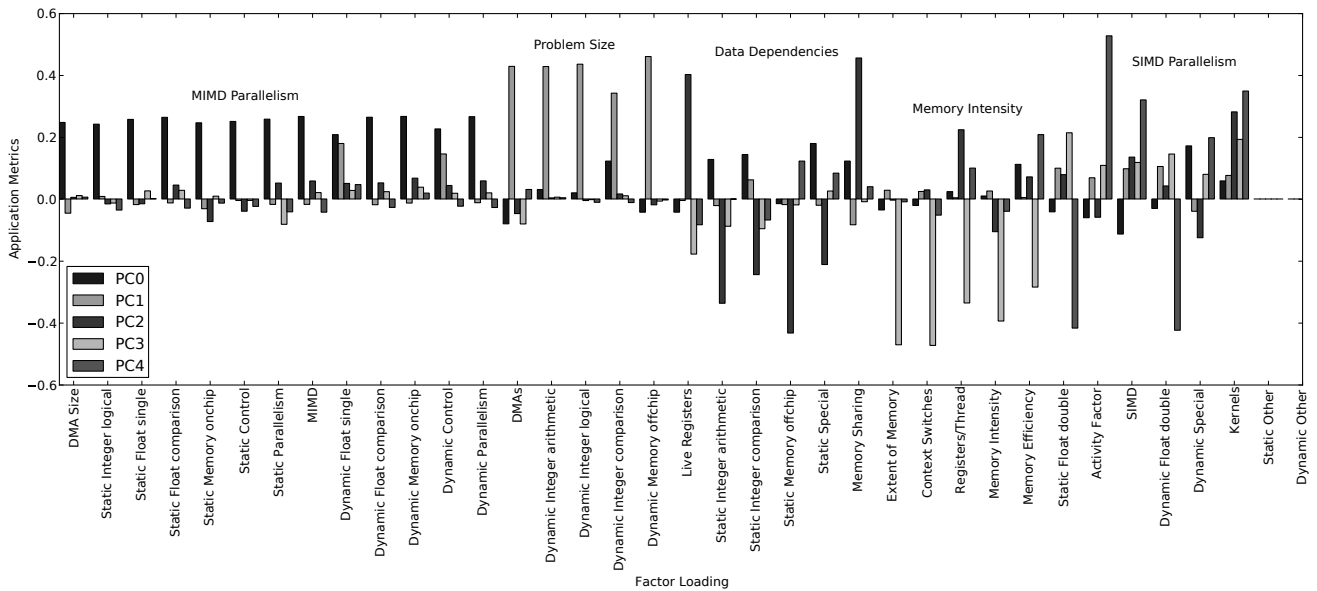
Figure 5: Factor loadings for the five application principal components. A factor loading closer to \pm 1 indicates a higher influence on the principal component.
