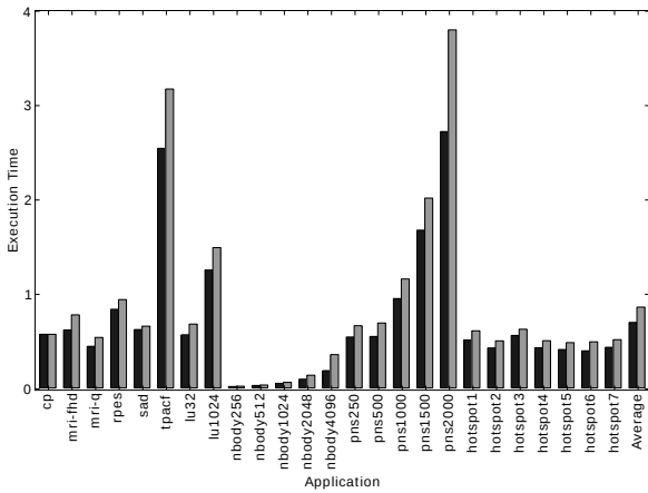
Figure 10: Predicted execution times for the 8800GTX using only static data and all other GPUs to train the model. Black indicates the measured time, and gray is the predicted time.
