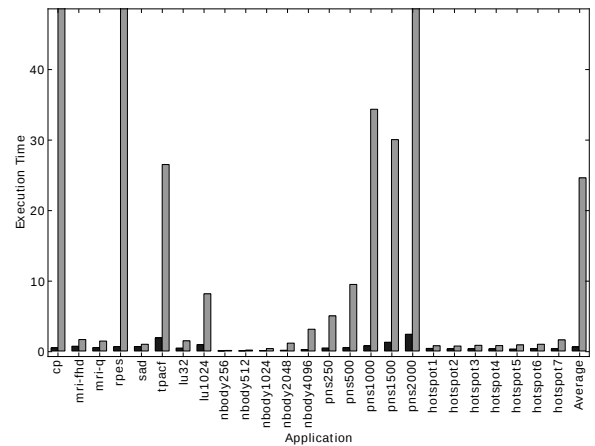
Figure 12: Predicted execution times for the 280GTX using all of the other processors for training. This is the least accurate model; it demonstrates the need for separate models for GPU and CPU architectures.
