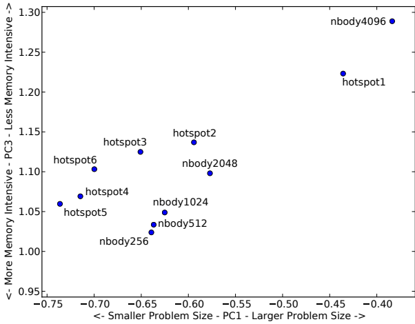
Figure 8: This figure shows the effect of increased problem size on the Memory Intensity of the Nbody and Hotspot applications. While this relationship probably will not hold in general, it demonstrates the usefulness of our methodology for characterizing the behavior of individual applications. We had originally expected these applications to become more memory intensive with an increased problem size; they actually become more compute intensive. This figure is also useful as a sanity check for our analysis, it correctly identifies the Nbody examples with higher body counts as having a larger problem size.
