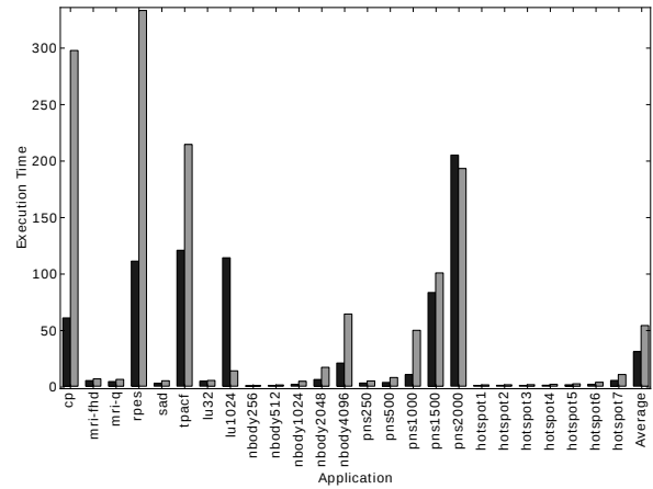
Figure 11: Predicted execution times for the AMD Phenom processor using the Atom and Nehalem chips for training.
