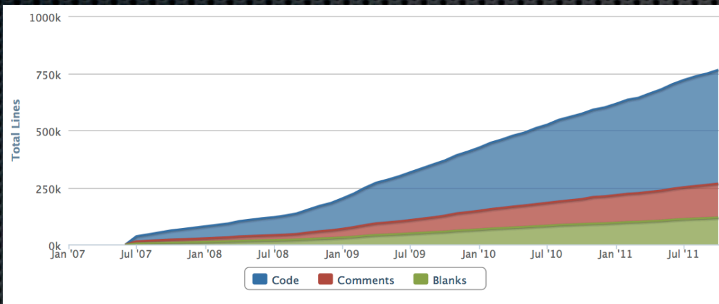
Clang LOC
