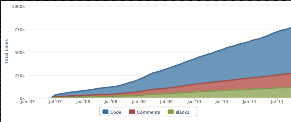
Clang LOC
